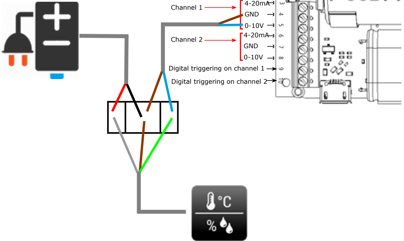
Temperature + humidity sensor
